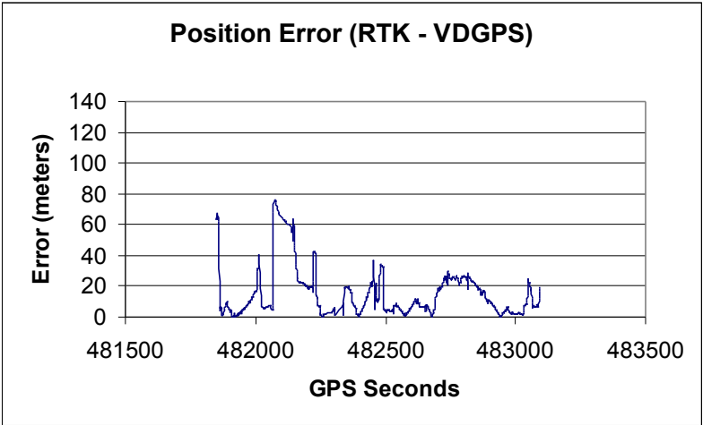
Figure 10. VDGPS Position Errors
